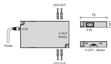
MEC Lite RP 150W
