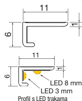
Profil s LED trakama
